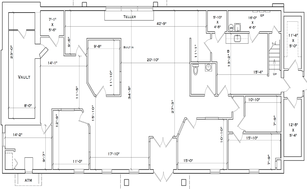
FIRST FLOOR 3,304 SQ. FT.
