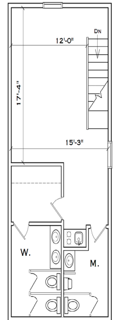
SECOND FLOOR 576 SQ. FT.
